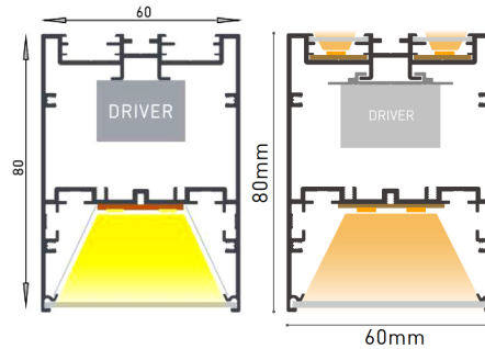
O—Opal smooth/1m, 18.4W
