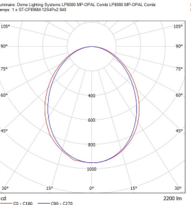
OP—Combined Opal Prism/1m, 18.4W
