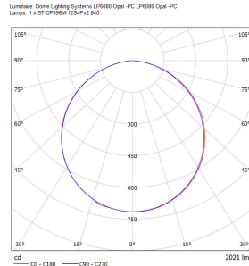
O—Opal smooth/1m, 18.4W
