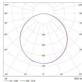
O—Opal smooth/1m, 18.4W Luminaire: Dome Lighting Systems LP6880 Opal-PC LP6880 Opal-PC Lamp: 1 x ST-CP6880M 1254P/2 840
