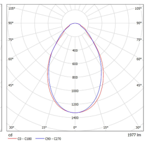
MP—2 Layer Prism (UGR19)/1m, 18.4W Luminaire: Dome Lighting Systems LP6880 M-Prism H.0.2mm LP6880 M-Prism H.0.2mm Lamp: 1 x ST-CP6880M 1254P/2 840
