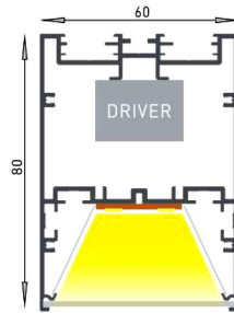
O—Opal smooth/1m, 18.4W Luminaire: Dome Lighting Systems LP6880 Opal-PC LP6880 Opal-PC Lamp: 1 x ST-CP6880M 1254P/2 840
