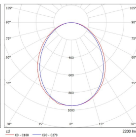
OP—Combined Opal Prism/1m, 18.4W Luminaire: Dome Lighting Systems LP6880 MP-OPAL Combi LP6880 MP-OPAL Combi Lamp: 1 x ST-CP6880M 1254P/2 840
