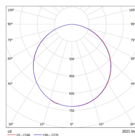
O—Opal smooth/1m, 18.4W Luminaire: Dome Lighting Systems LP8080 Opal-PC LP8080 Opal-PC Lamps: 1 x ST-CP8580M 125SPx2 840
