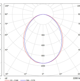
OP—Combined Opal Prism/1m, 18.4W Luminaire: Dome Lighting Systems LP8080 MP-OPAL Combi LP8080 MP-OPAL Combi Lamps: 1 x ST-CP8580M 125SPx2 840
