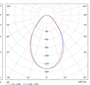
MP—2 Layer Prism (UGR19)/1m, 18.4W Luminaire: Dome Lighting Systems LP8080 M-Prism H.L.0.2mm LP8080 M-Prism H.L.0.2mm Lamps: 1 x ST-CP8580M 125SPx2 840
